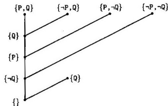
Figure 5.2 Chain of resolutions in a linear deduction.
